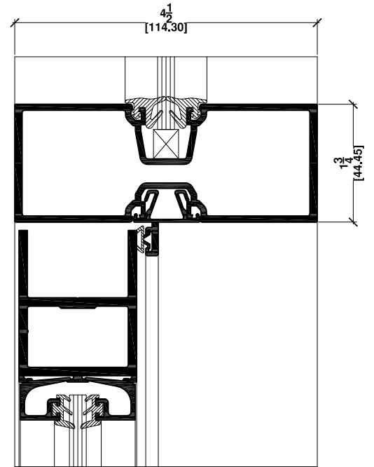
4b HOR. MULLION FIXED GLASS/S175 DOOR TWO POCKET MULL.
