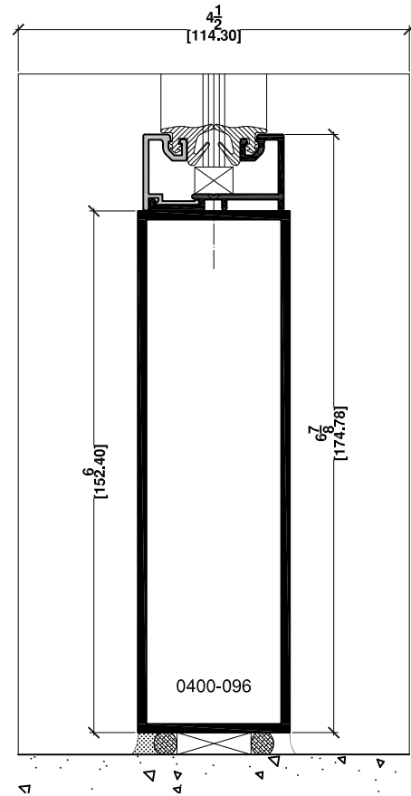
3g SILL FIXED GLASS 6" PLAIN TUBE
