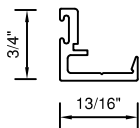
PART #: 450-235 DOOR STOP BASE USE FOR GEAR CONTINUOUS HINGE
