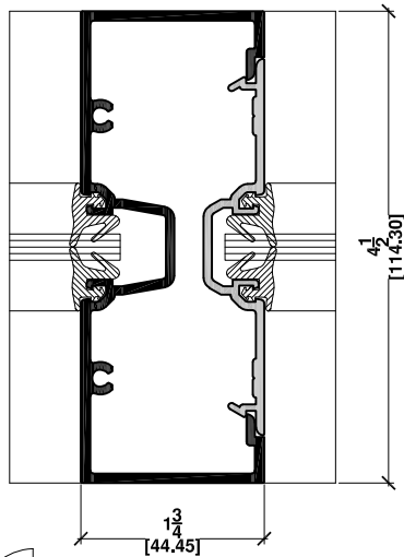
13 VERT. MULLION FIXED GLASS - FIXED GLASS O/B MULL. W/ADAPTOR
