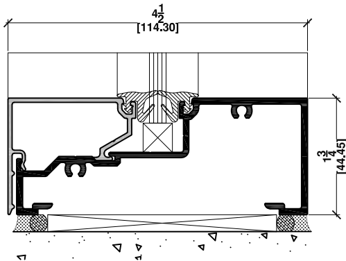
3 SILL FIXED GLASS SILL O/B
