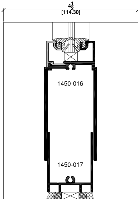
3b SILL FIXED GLASS ADJUST. SIDELITE MULL.
