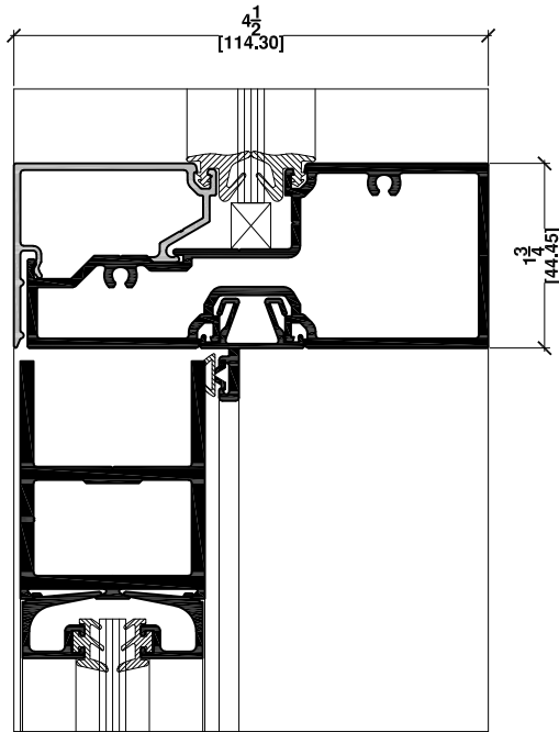
4 HOR. MULLION FIXED GLASS/ SERIES 175 DOOR
