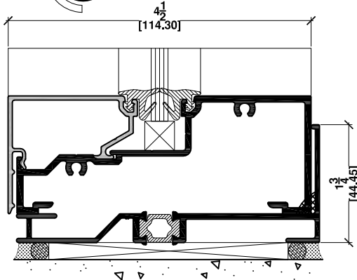
3d SILL FIXED GLASS/HOR. MULL. W/ SILL BASE O/B
