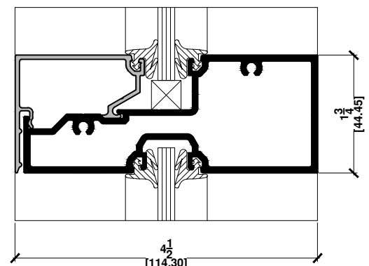
2 HOR. MULLION FIXED GLASS/FIXED GLASS
