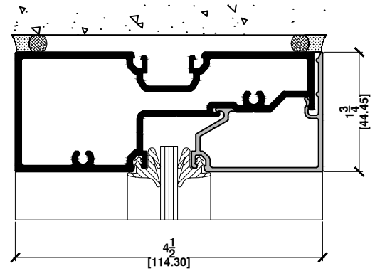
1c HEAD FIXED GLASS HOR. MULLION
