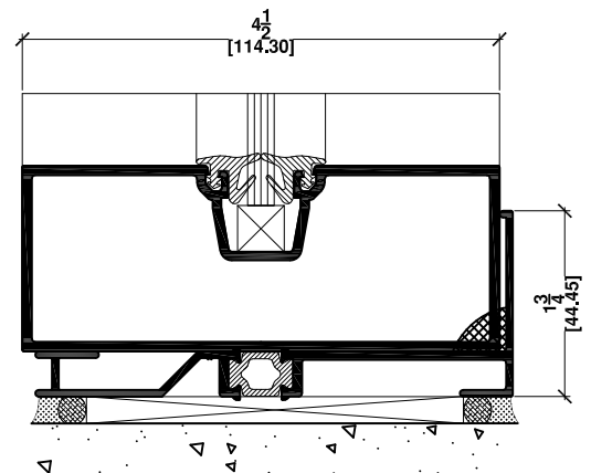
3i SILL W/ SILL BASE FIXED GLASS/HOR. MULL. ONE POCKET MULL. O/B
