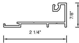
PART #: 1450-022 GLASS STOP BASE FOR 1" (25mm) SEALED UNIT
