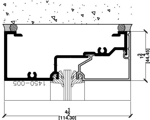
1b HEAD FIXED GLASS
