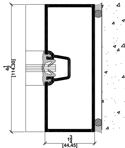
14a JAMB FIXED GLASS O/B MULL. W/ADAPTOR
