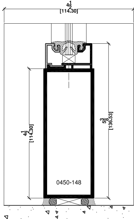
3f SILL FIXED GLASS 4 1/2" PLAIN TUBE
