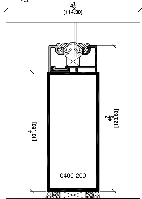
3c SILL FIXED GLASS 4" PLAIN TUBE
