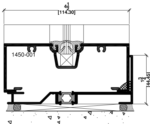
3h SILL W/ SILL BASE FIXED GLASS/HOR. MULL. ONE POCKET MULL. C/B
