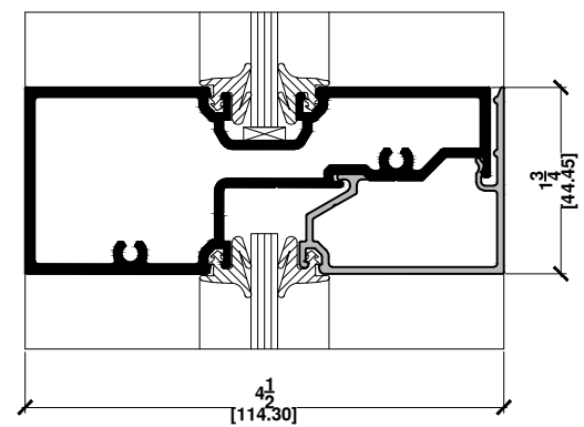
2a HOR. MULLION FIXED GLASS/FIXED GLASS
