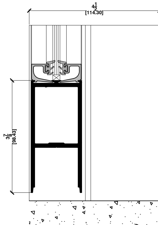
SERIES 175 DOOR W/O THRESHOLD
