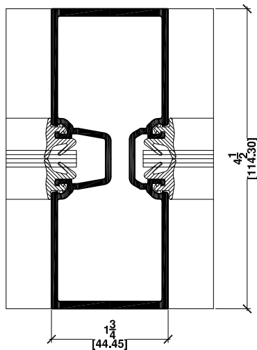
13a VERT. MULLION FIXED GLASS - FIXED GLASS TWO POCKET MULL.
