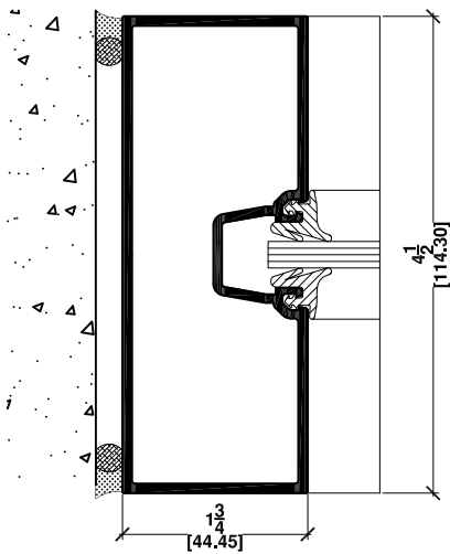
6 JAMB FIXED GLASS ONE POCKET MULL. C/B
