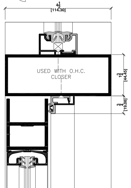
4b HOR. MULLION FIXED GLASS/S175 DOOR TWO POCKET MULL.
