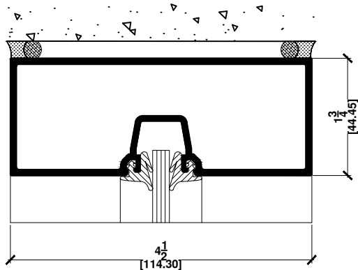
1a HEAD FIXED GLASS ONE POCKET MULL. C/B
