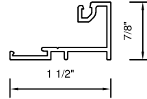
PART #: 1450-020 GLASS STOP BASE FOR 1/4" (6mm) GLASS
