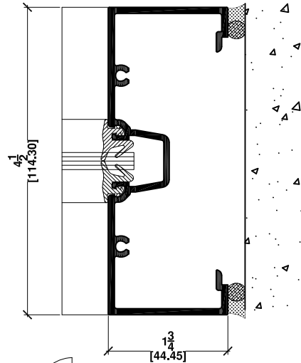
14 JAMB FIXED GLASS ONE POCKET MULL. O/B
