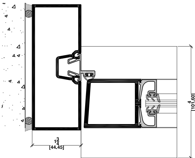
8 JAMB ONE POCKET MULL. C/B - SERIES 175 DOOR
