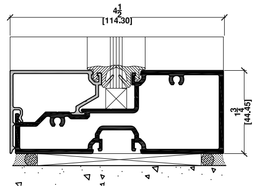
3e SILL FIXED GLASS HOR. MULLION
