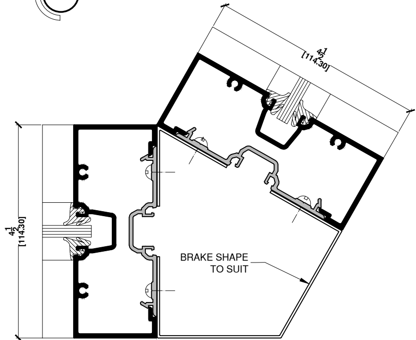
12a VERT. MULLION FIXED GLASS - FIXED GLASS 120° OUTSIDE CORNER
