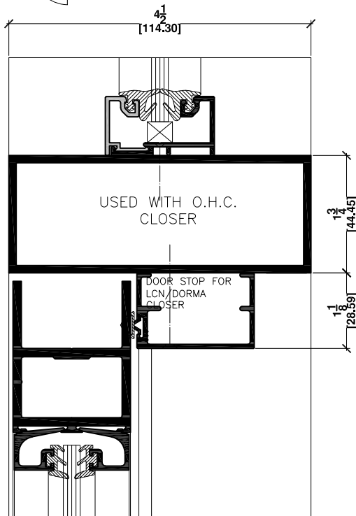
4 HOR. MULLION FIXED GLASS/ SERIES 175 DOOR
