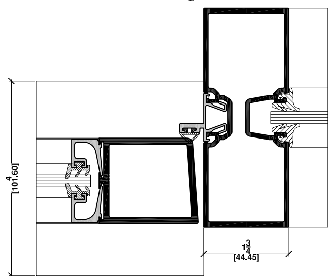
9 VERT. MULLION SERIES 175 DOOR - TWO POCKET MULL.
