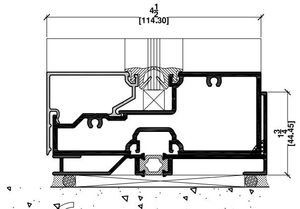
3a SILL FIXED GLASS/HOR. MULL. W/ SILL BASE C/B
