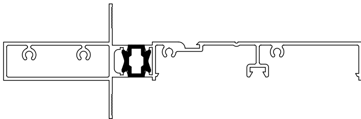
PART #: 612-714 PERIMETER WITH MULLION FACE 7" (177.8mm) USE 1/8" GLAZING TAPE
