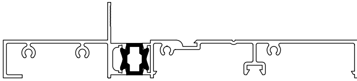
PART #: 612-701 FRAME PERIMETER 7" (177.8mm) USE 1/8" GLAZING TAPE
