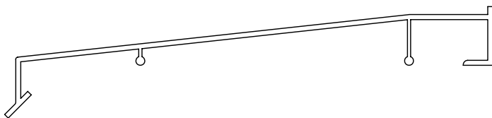
PART #: 411-006 SILL 6-3/4" (171.5mm) USE UNDER WINDOW FRAME
